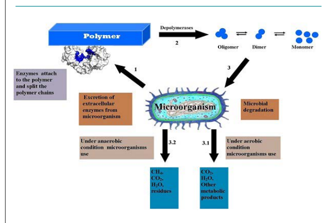
Figure 2. General Mechanism of Plastic Biodegradation Under Aerobic and Anaerobic Conditions. 23
