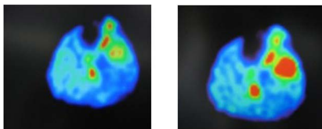
Figure 2. The Depicted Figure Shown The Evidence of Glucose Uptake in Primary Lung Cancer Tissue and Also Correlated with Size Dependent in c-myc Treated by DEN at Age of 8.5-months or After 4.5-Months After End of Treatment
