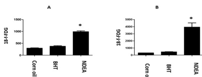
Figure 3. The Depicted Figure Shown the Highest Glucose Uptake (means±se) in Liver Harbor HCC in the Last Sacrifice after DEN Treatment at Age of 8.5-months (B). Notably, DEN Treated Transgenic Mice of Both First (A) and Last Sacrifice (B) Displayed a Significant Increase of Glucose Uptake when Compared with Transgenic Mice Treated by BHT or Corn Oil as Vehicle Groups
