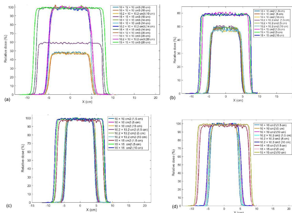
Figure 4. Comparison Beam Profile for Variation Field Size of 10 \times 10 \text{ cm}^2 , 10.2 \times 10.2 \text{ cm}^2 , 15 \times 15 \text{ cm}^2 , energy 6 MV, SSD 100 cm, Variation in the Target (a) Volume in Depth 10 cm with Variation Position of 10 cm, 14 cm, 20 cm, (b) Depth Variation of 1, 5 cm, 5 cm, 10 cm with Variation Position 10 cm, (c) 14 cm, (d) 20 cm
