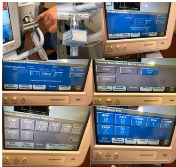
Figure 1. Add 2 HEPA Filters, One Immediately Connected to the V60 Main Gas Port Outlet and the Second HEPA Gets Connected to the Exhalation Valve Port Closer to the ET/Trach. To Connect to an ETT Tube You Need to Use the Philips Respironics Conventional Exhalation Valve and/or Circuit Kit. We Recommend that the HEPA Filter on the Exhalation Valve Port be Connected to a Blind Reservoir. Turn on Machine and Hit the Menu Tab. Please Ensure the Patient is not Connected to the V60 Machine
