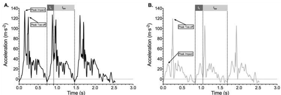
Figure 2: Accelerometer output for total accelerations (XYZ-planes) versus time (s) at the foot for the LTM (A) and ATM (B) conditions. Ground contact ( t_c ) and swing time ( t_{sw} ) are highlighted along with peak impact and peak toe-off.
