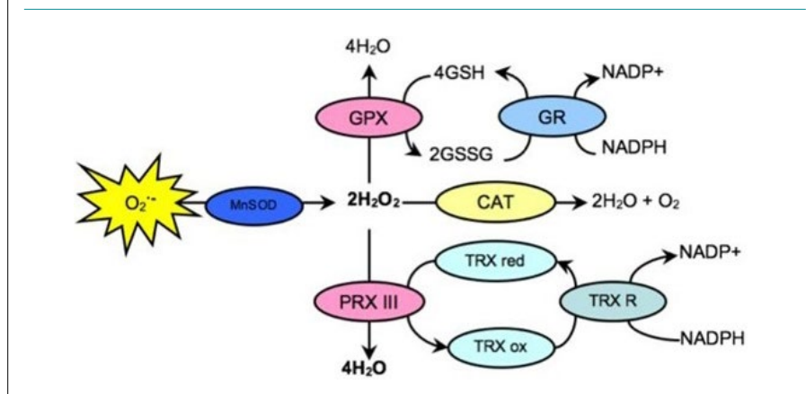
Figure 1. Simplistic Overview of the Interaction of Antioxidant Enzyme Network in Mitochondria: A super oxide radical ( O_2^- ) produced from mitochondria is converted into hydrogen peroxide ( H_2O_2 ), which is then detoxified by several antioxidant enzymes such as glutathione peroxidase (GPX), catalase (CAT), and peroxiredoxin III (PRX III), resulting in the conversion of H_2O_2 into water molecules. Importantly, GPX and PRX III utilize reducing molecules such as glutathione and reduced thioredoxin (TRX red), respectively to neutralize H_2O_2 . After donating thiol groups, oxidized glutathione (GSSG) and thioredoxin (TRX ox) become reduced by glutathione reductase (GR) and thioredoxin reductase (TRX R), respectively, using NADPH as a reducing equivalent.
