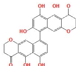
chaetochromin (23)
