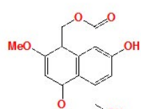
corymbiferan lactone I (26)
