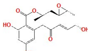
5'-hydroxymonocillin (20)
