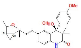
aspoquinolone II (52) 20 (R); 21 (S)
