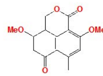
corymbiferan lactone IV (29)
