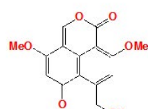
corymbiferan lactone III (28)
