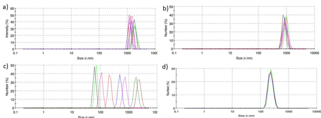
Figure 2. DLS Analysis of the Average Particle Size (d, nm) of each Conjugate. The DLS Spectra Show the Size Distribution of (a) Conjugate 5, (b) Conjugate 6, (c) Conjugate 7, and (d) Conjugate 8
