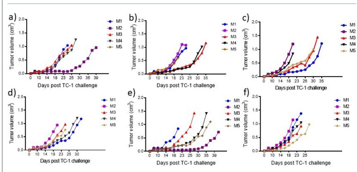
Figure 4. Vaccine Immunotherapeutic Effect on the Change in Tumor Volume for each Mouse. The Tumor Volume ( \text{cm}^3 ) in Individual Mice Treated with (a) Physical Mixture of 8Q_{\min} and ISA51, (b) PBS, (c) Conjugate 5, (d) Conjugate 6, (e) Conjugate 7, and (f) Conjugate 8 were Measured from Day 0 to the Day that Mouse was Culled
