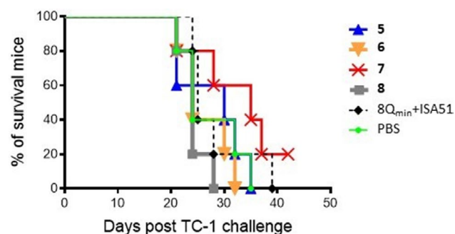
Figure 5. Survival Rates of Mice. The Survival Rate of each Group of Mice was Recorded from Day 0 to Day 44, when the Last Mouse was Culled
