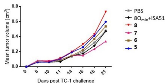
Figure 3. Mean Tumor Volume (Cm3) of Mice Challenged with 5×10 5 Tc-1 Cells/Mouse (Day 0), Then immunized on Day 7 with Compound 5, 6, 7, or 8, or Positive/Negative Control Solution
