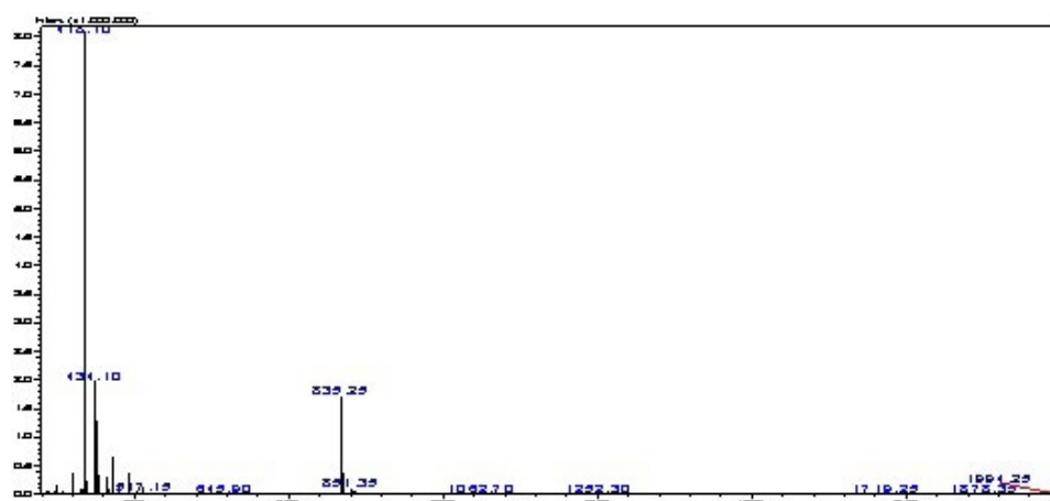
Figure S1. Mass Spectrum of Fmoc-Dhc-Oh
