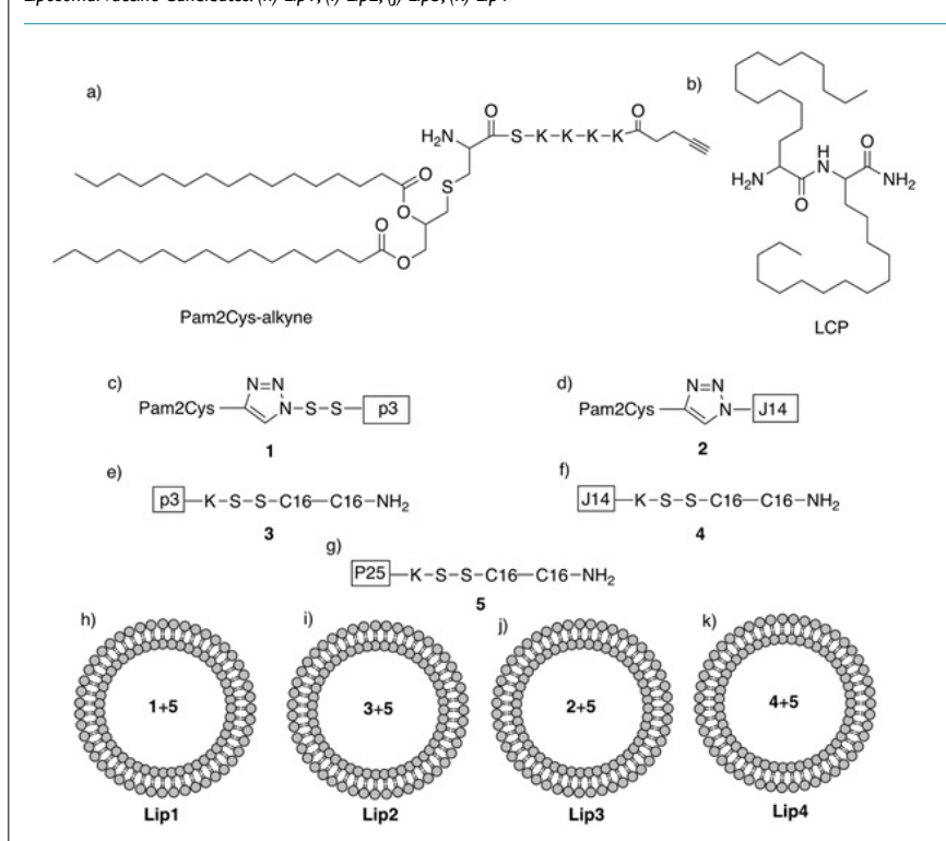
Figure 1. Schematic Representation of the Vaccine Candidates. Lipids: (a) Pam2CysSKKKK-alkyne (Pam2Cys-alkyne), (b) LCP (C16-C16); Lipopeptides: (c) 1 (Pam2Cys-p3), (d) 2 (Pam2Cys-J14), (e) 3 (p3-LCP), (f) 4 (J14-LCP), (g) 5 (P25-LCP); Liposomal Vaccine Candidates: (h) Lip1, (i) Lip2, (j) Lip3, (k) Lip4
