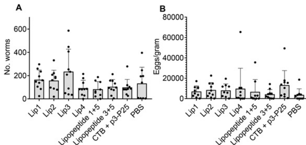
Figure 8. Parasite (adult worm and egg) Burden were Analyzed 7 Days Post-infection with Nippostrongylus Brasiliensis
