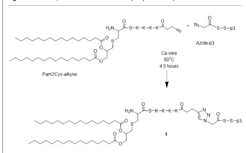
Figure 5. Schematic of the Click Reaction between Pam2Cys-alkyne and azide-p3
