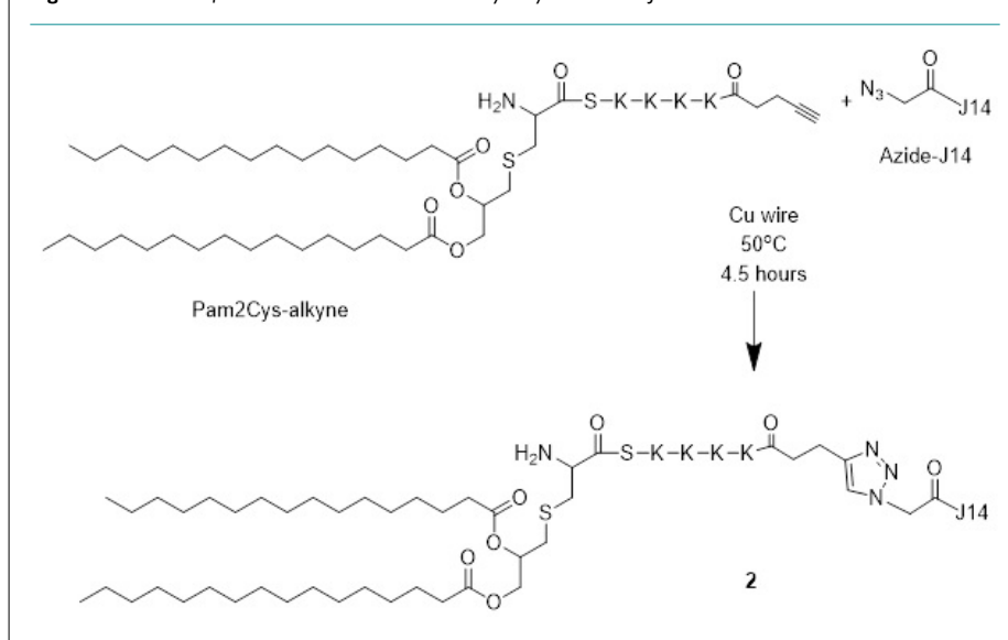
Figure 6. Schematic of the Click Reaction between Pam2Cys-alkyne and azide-J14
